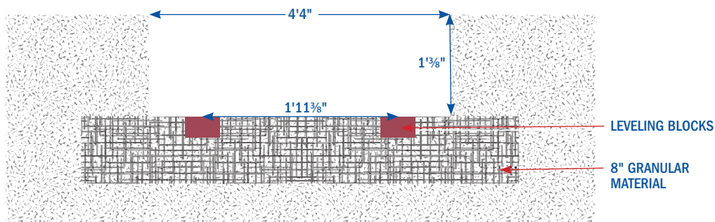
FRONT CROSS-SECTION
