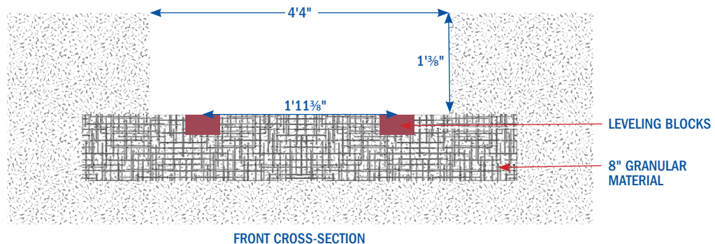
FRONT CROSS-SECTION
